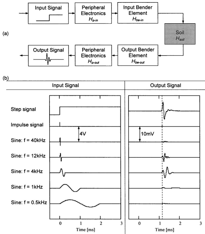
Fig. 7. Bender element installation: (a) sequence of frequency response functions; and (b) input and output signals. Tip-to-tip distance: L=105 mm, cantilever length: 6.5 mm, V_S=93 m/s. Resonant frequency of bender element f_r=3.6 kHz, L/\lambda=4.0 .
