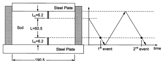
Fig. 9. Multiple-reflection method. All dimensions are in millimeters.
