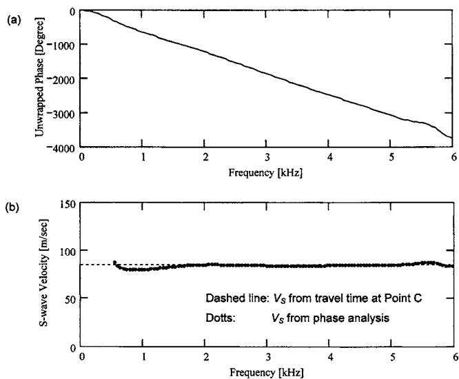
Fig. 11. Phase analysis in multiple reflection method: (a) unwrapped phase; and (b) S-wave velocity spectrum
