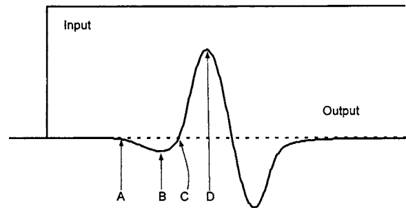
Fig. 8. Typical S-wave signal within near field ( L/\lambda=1 ): (A) first deflection, (B) first bump maximum, (C) zero after first bump, and (D) major first peak
