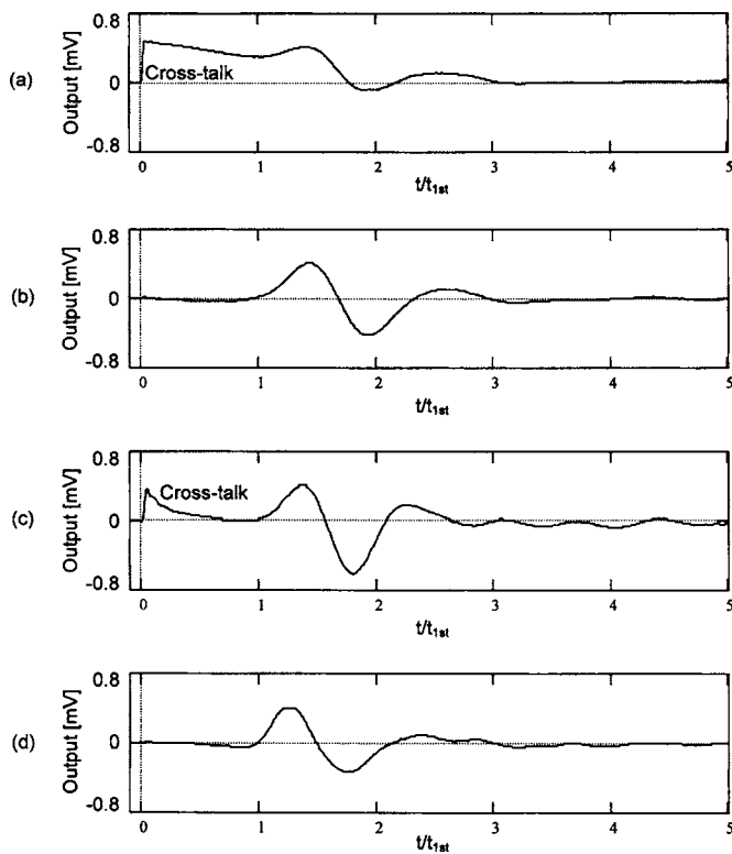
Fig. 2. Crosstalk effects: (a) series-to-series without grounding; (b) series-to-series with shielding and grounding; (c) parallel-to-series without shielding and grounding; and (d) parallel-to-parallel without shielding. Time “ t_{1st} ” corresponds to S-wave first arrival (input: step signal, tip-to-tip distance: L=100 mm).
