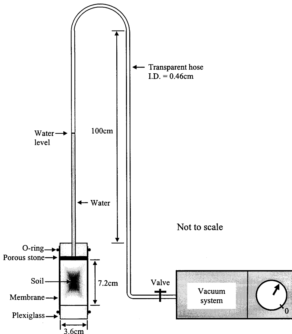
FIG. 1—Device and experimental setup used for the simple CS test.
