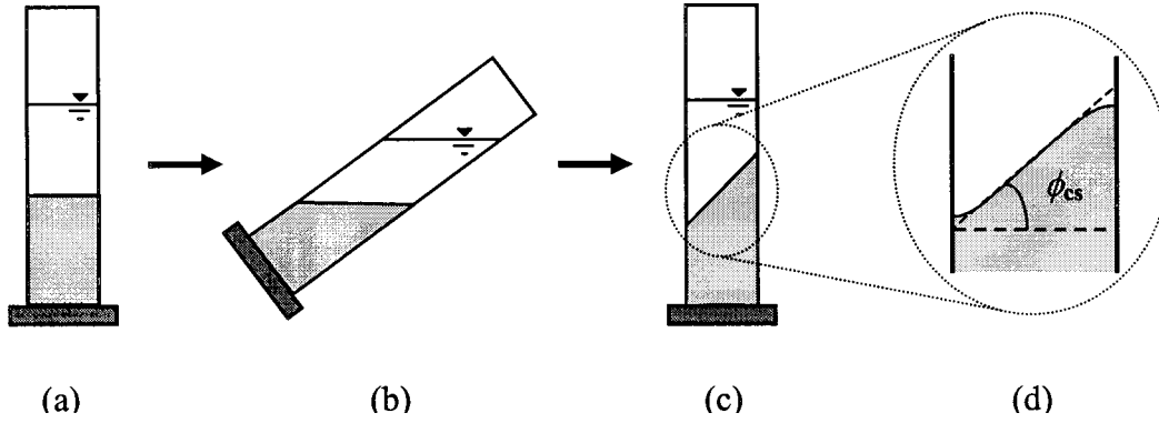
FIG. 2—Simplified method to determine the critical state friction angle: (a) Pour soil in a 1000-mL cylinder with water. (b) Rotate the cylinder passed 60°. (c) Slowly return the cylinder to its vertical position and measure the angle of repose. (d) The angle is measured in the middle region of the slope.
