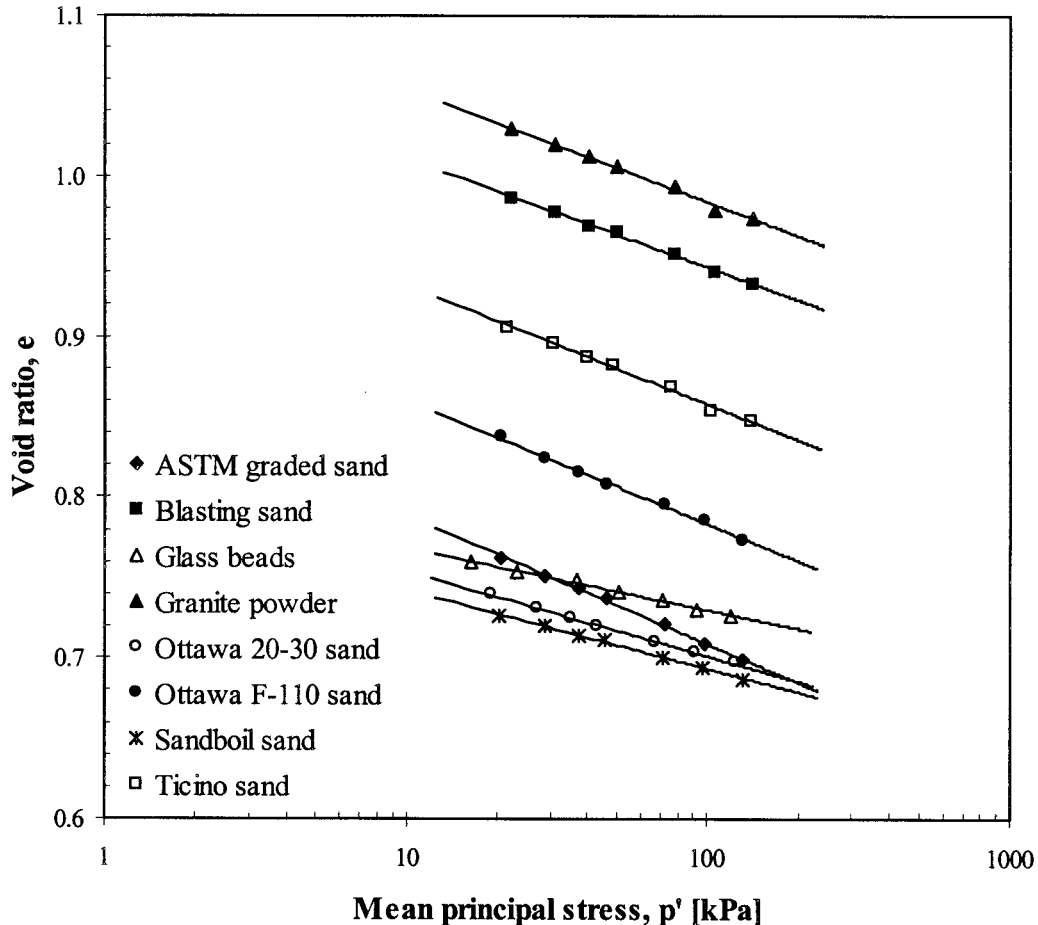
FIG. 4—Simple CS test results— e - \log p' projection of the critical state line for the different soils.
