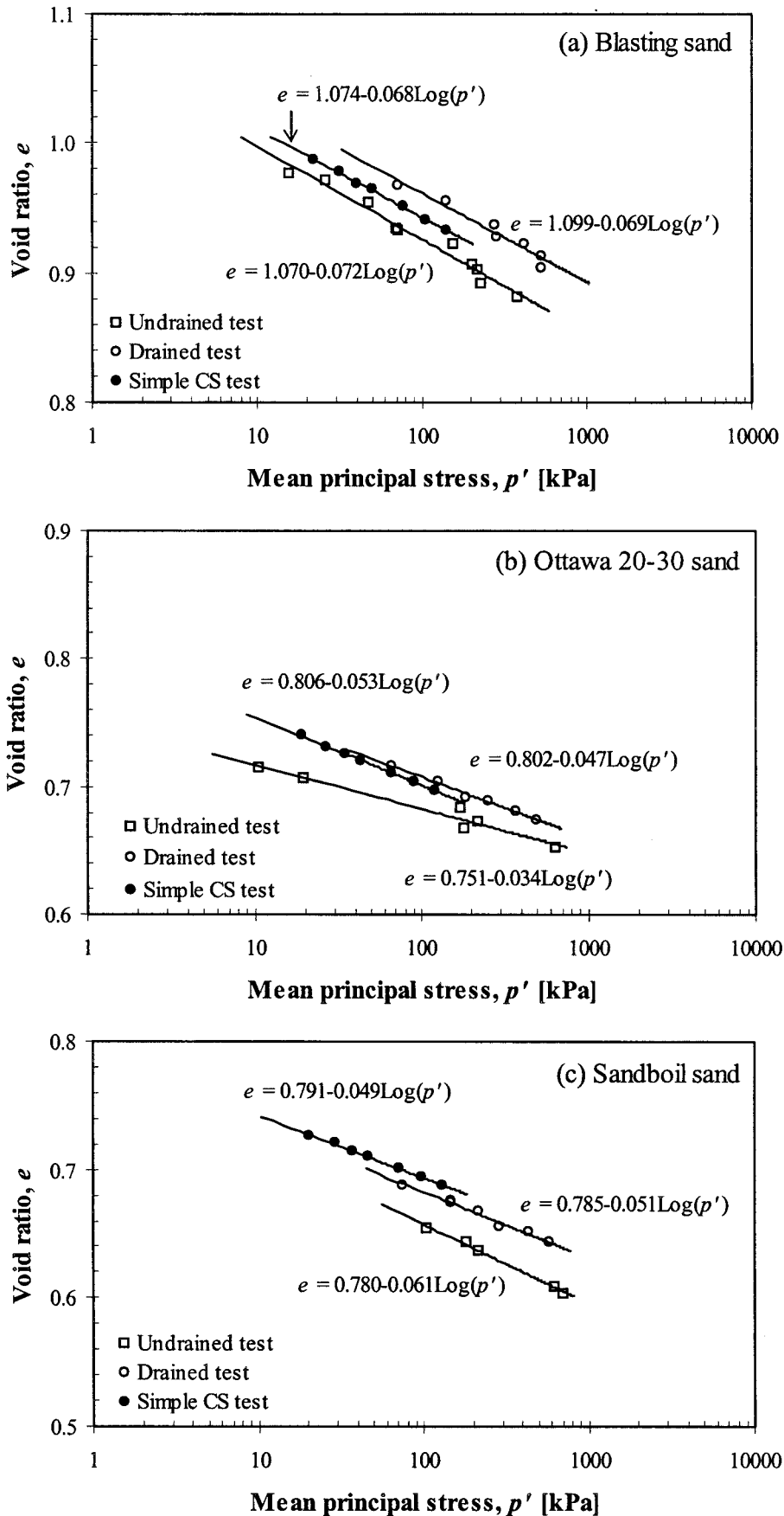
FIG. 5—Comparison between simple CS test results and triaxial test results.
